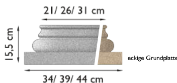
proKERA SANDLINE BAS-I8 a Ø 20 cm BAS-8 a BAS-I8 b Ø 25 cm BAS-8 b BAS-I8 c Ø 30 cm BAS-8 c
