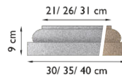
proKERA SANDLINE BAS-I6 a Ø 20 cm BAS-6 a BAS-I6 b Ø 25 cm BAS-6 b BAS-I6 c Ø 30 cm BAS-6 c
