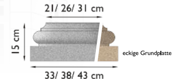
proKERA SANDLINE BAS-I6 a Ø 20 cm BAS-6 a BAS-I6 b Ø 25 cm BAS-6 b BAS-I6 c Ø 30 cm BAS-6 c
